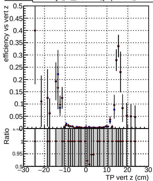
Efficiency vs vert z — DQM_TT_ORIGINAL — DQM_TT_MODIFIED_propToPlane_PVersionFINAL2 — DQM_TT_MODIFIED_propToPlane_PVersionFINAL3
