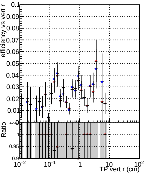
Efficiency vs vertpos DQM_TT_ORIGINAL DQM_TT_MODIFIED_propToPlane_PRVersionFINAL2 DQM_TT_MODIFIED_propToPlane_PRVersionFINAL3
