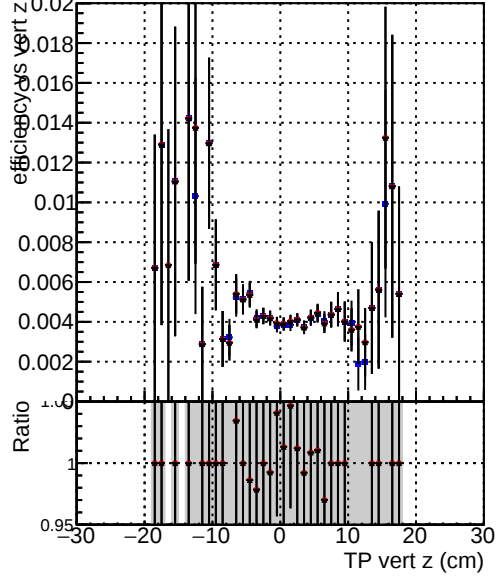
Efficiency vs. TP vert z —●— DQM_TT_ORIGINAL —●— DQM_TT_MODIFIED_propToPlane_PRRVersionFINAL2 —●— DQM_TT_MODIFIED_propToPlane_PRRVersionFINAL3
