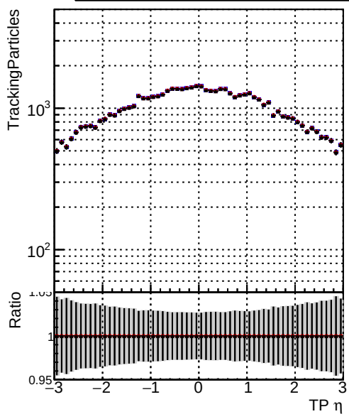
N of simulated tracks vs eta Legend: DQM_TT_ORIGINAL (blue line with dots) DQM_TT_MODIFIED_propToPlane_PVersionFINAL2 (red line with dots) DQM_TT_MODIFIED_propToPlane_PVersionFINAL3 (black line with dots)
