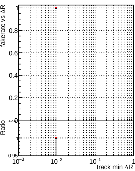
Fake rate vs \Delta R(\text{track, jet}) DQM TT ORIGINAL DQM TT MODIFIED_propToPlane_FINAL2 DQM TT MODIFIED_propToPlane_FINAL3
