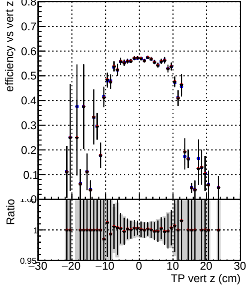
Efficiency vs. TP vert z (cm) Legend: - DQM_TT_ORIGINAL (blue stars) - DQM_TT_MODIFIED_propToPlane_PRRVersionFINAL2 (red stars) - DQM_TT_MODIFIED_propToPlane_PRRVersionFINAL3 (black stars)
