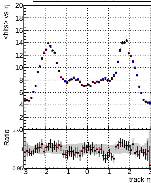
mean hits vs \eta — DQM_TT_ORIGINAL — DQM_TT_MODIFIED_propToPlane_PRRVersionFINAL2 — DQM_TT_MODIFIED_propToPlane_PRRVersionFINAL3
