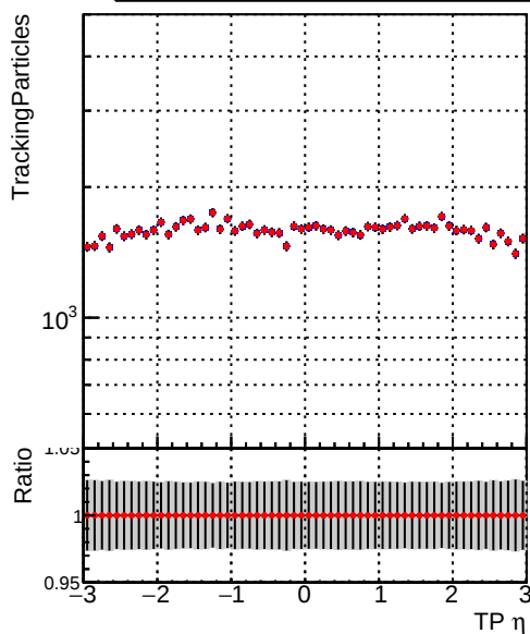
Legend: DQM_TT_ORIGINAL (blue line), DQM_TT_MODIFIED_propToPlane_PRVersionFINAL2 (red line)
