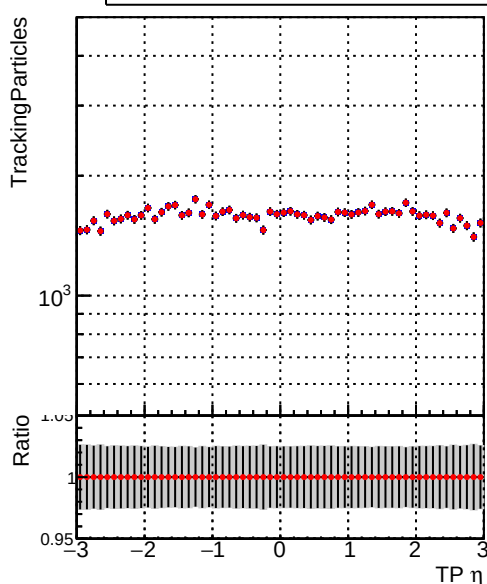
N of simulated tracks vs TP \eta —•— DQM_TT_ORIGINAL —•— DQM_TT_MODIFIED_propToPlane_PRVersionFINAL2
