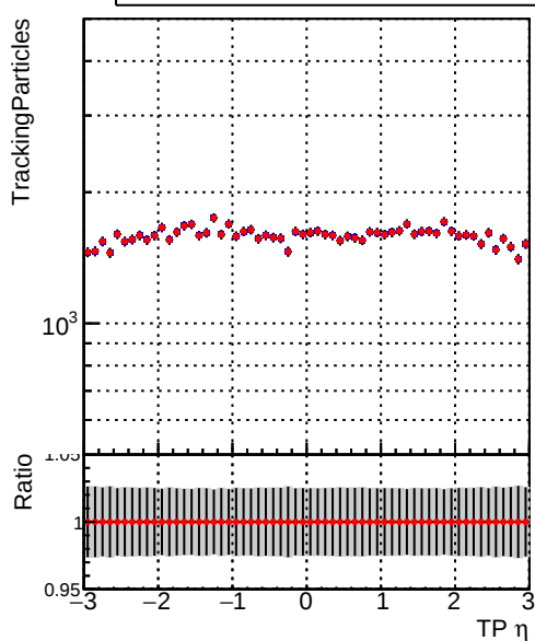
N of simulated tracks vs TP \eta Legend: DQM_TT_ORIGINAL (blue squares), DQM_TT_MODIFIED_propToPlane_PRVersionFINAL2 (red circles)
