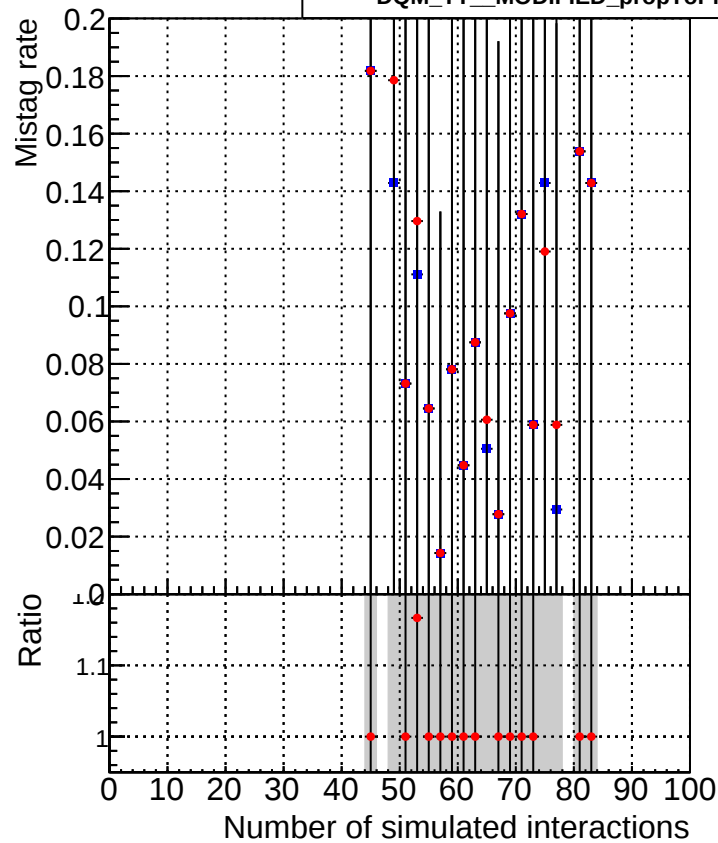
—■ DQM_TT_ORIGINAL —● DQM_TT_MODIFIED_propToPlane_PRVersionFINAL2
