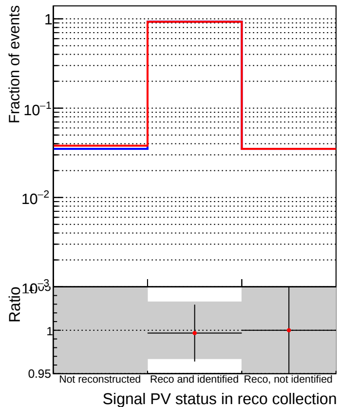
—■ DQM_TT_ORIGINAL —● DQM_TT_MODIFIED_propToPlane_PRVersionFINAL2
