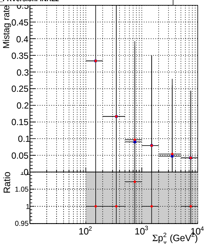
—■ DQM_TT_ORIGINAL —● DQM_TT_MODIFIED_propToPlane_PRVersionFINAL2
