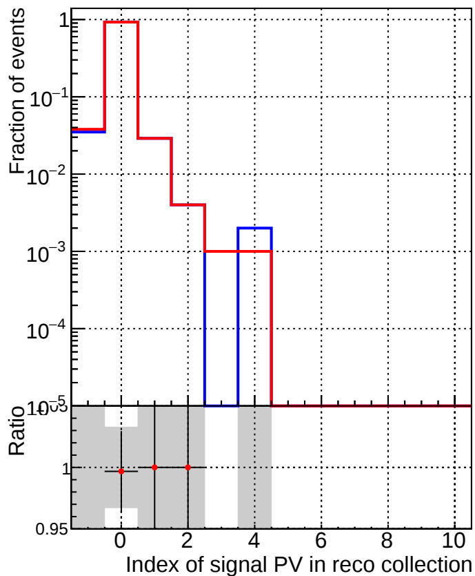
—■ DQM_TT_ORIGINAL —● DQM_TT_MODIFIED_propToPlane_PRVersionFINAL2
