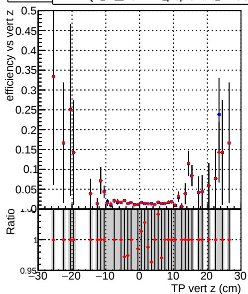
Efficiency vs. TP vert z (cm) Legend: —●— DQM_TT_ORIGINAL, —●— DQM_TT_MODIFIED_propToPlane_PRVersionFINAL2
