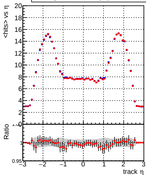
mean hits vs \eta Legend: DQM_TT_ORIGINAL (blue line), DQM_TT_MODIFIED_propToPlane_PRVersionFINAL2 (red line with error bars)
