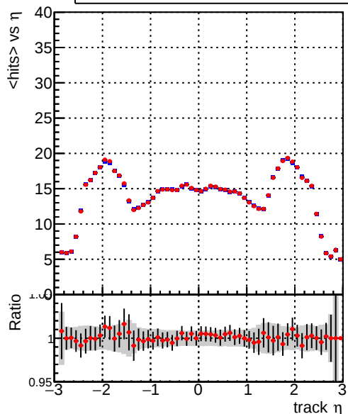
mean hit — DQM_TT_ORIGINAL — DQM_TT_MODIFIED_propToPlane_PRVersionFINAL2
