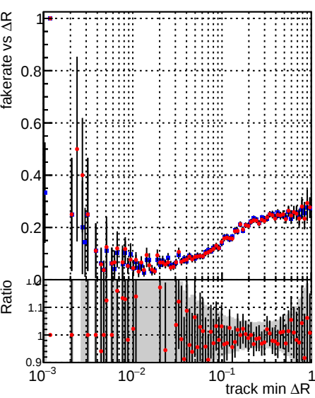
Legend: DQM_TT_ORIGINAL (blue squares), DQM_TT_MODIFIED_propToPlane_PRVersionFINAL2 (red stars)
