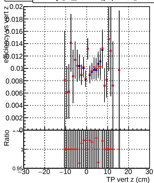
Efficiency vs. TP vert z (cm) — DQM_TT_ORIGINAL — DQM_TT_MODIFIED_propToPlane_PRVersionFINAL2
