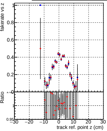
Fake rate vs v DQM_TT_ORIGINAL DQM_TT_MODIFIED_propToPlane_PRVersionFINAL2
