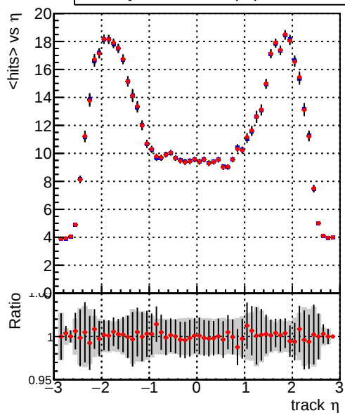
mean hits vs \eta Legend: DQM_TT_ORIGINAL (blue line with markers), DQM_TT_MODIFIED_propToPlane_PRVersionFINAL2 (red line with markers)
