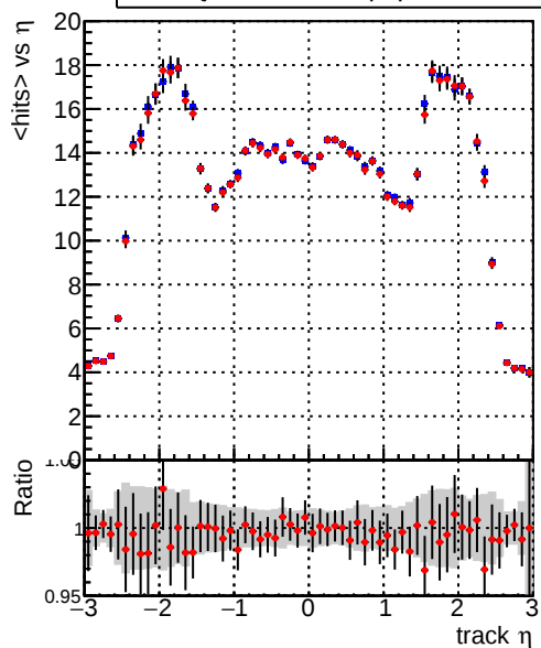
mean hits vs \eta Legend: DQM_TT_ORIGINAL (Blue line), DQM_TT_MODIFIED_propToPlane_PRVersionFINAL2 (Red line)
