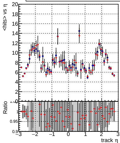
mean hit Legend: DQM_TT_ORIGINAL (blue line with circles), DQM_TT_MODIFIED_propToPlane_PRVersionFINAL2 (red line with circles)
