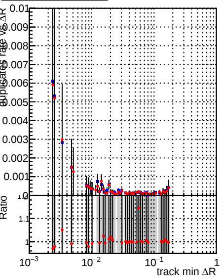
Legend: DQM_TT_ORIGINAL (grey bars), DQM_TT_MODIFIED_propToPlane_PRVersionFINAL2 (red dots)
