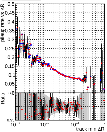
Legend: DQM_TT_ORIGINAL (grey bars), DQM_TT_MODIFIED_propToPlane_PRVersionFINAL2 (red dots)
