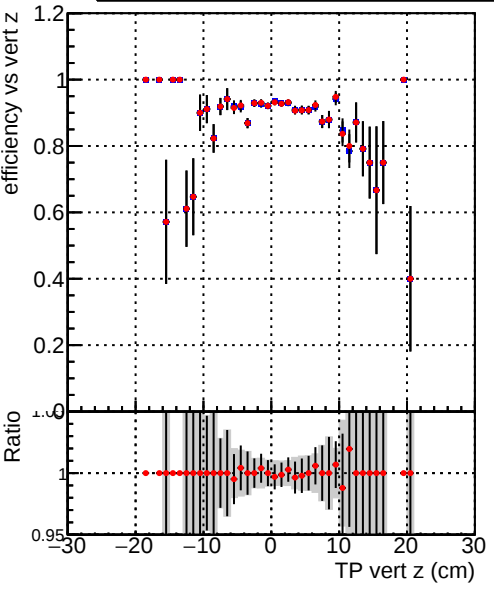
Efficiency vs TP vert z (cm) Legend: DQM_TT_ORIGINAL (blue squares) DQM_TT_MODIFIED_propToPlane_PRVersioFINAL2 (red diamonds)
