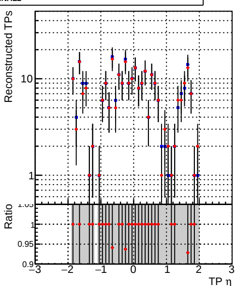
N of associated tracks (simToReco) vs TP η
