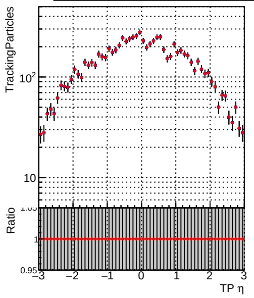
Legend: DQM_TT_ORIGINAL (blue squares), DQM_TT_MODIFIED_propToPlane_PRVersionFINAL2 (red diamonds)
