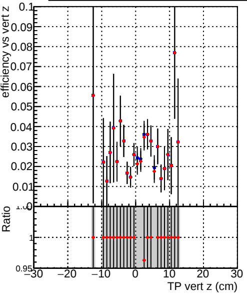
Efficiency vs vertpos Legend: DQM_TT_ORIGINAL DQM_TT_MODIFIED_propToPlane_PRVersionFINAL2
