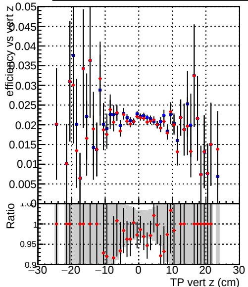
Efficiency vs vert z — DQM_TT_ORIGINAL — DQM_TT_MODIFIED_propToPlane_PRVersionFINAL2
