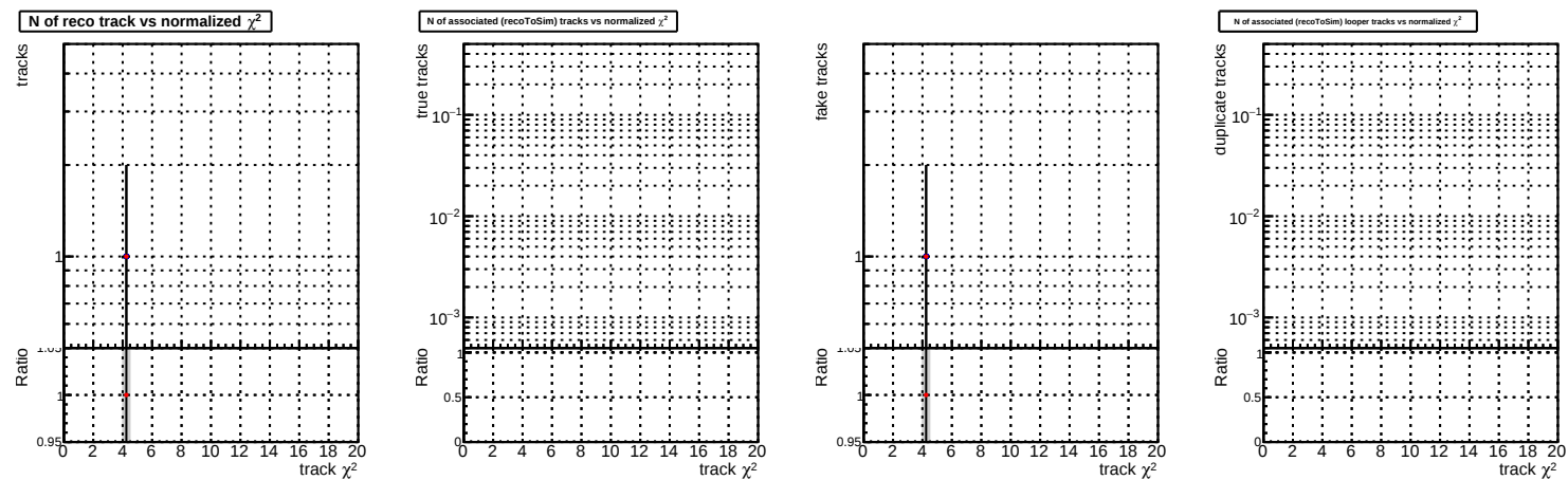
N of reco track vs. \chi^2 for DQM TT ORIGINAL (blue line) and DQM TT MODIFIED_propToPlane_PRVersionFINAL2 (red line).
