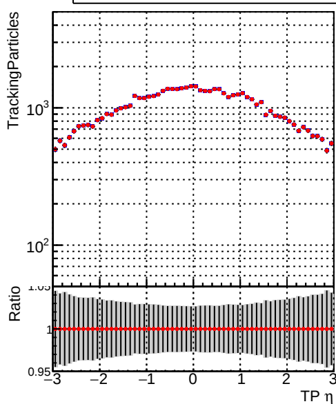
N of simulated tracks vs \eta Legend: DQM_TT_ORIGINAL (blue squares), DQM_TT_MODIFIED_propToPlane_PRVersionFINAL2 (red diamonds)
