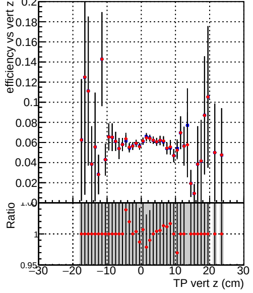
Efficiency vs. TP vert z — DQM_TT_ORIGINAL — DQM_TT_MODIFIED_propToPlane_PRRVersionFINAL2
