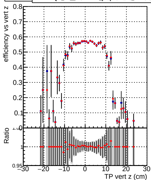
Efficiency vs. TP vert z (cm) — DQM_TT_ORIGINAL — DQM_TT_MODIFIED_propToPlane_PVVersionFINAL2
