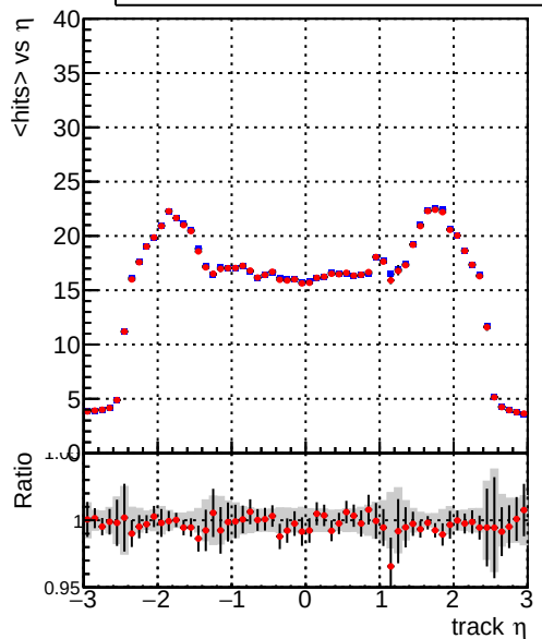
mean hits vs \eta — DQM_TT_ORIGINAL — DQM_TT_MODIFIED_propToPlane_PRVersionFINAL2
