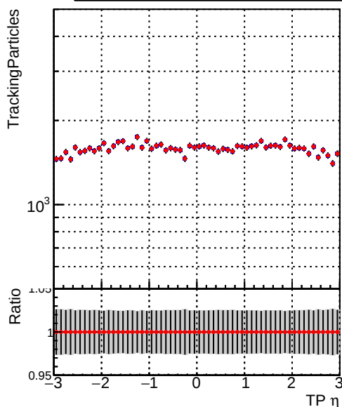
Legend: DQM_TT_ORIGINAL (blue dots), DQM_TT_MODIFIED_propToPlane_PRVersioniFINAL (red dots)
