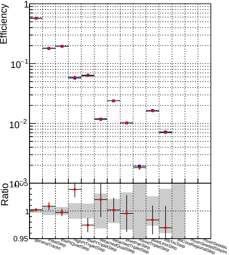
DQM_TT_ORIGINAL DQM_TT_MODIFIED_propToPlane_PRRVersioniFINAL
