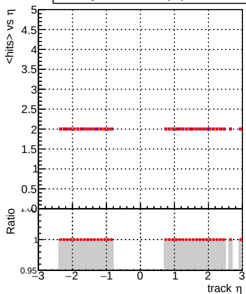
mean hits Legend: DQM_TT_ORIGINAL (blue line), DQM_TT_MODIFIED_propToPlane_PRVersionFINAL (red line)
