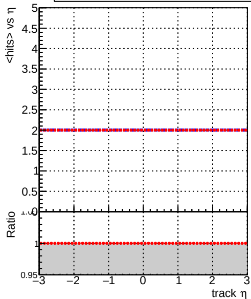
mean hit — DQM_TT_ORIGINAL — DQM_TT_MODIFIED_propToPlane_PRVersioniFINAL
