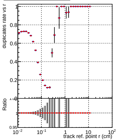
—•— DQM_TT_ORIGINAL —•— DQM_TT_MODIFIED_propToPlane_PRVersioniFINAL
