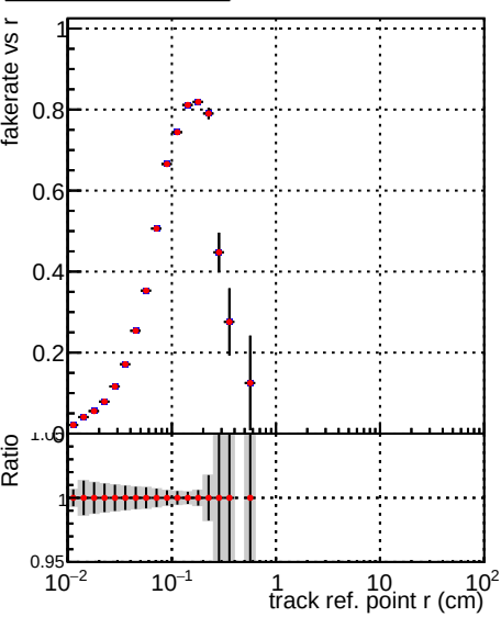
—•— DQM_TT_ORIGINAL —•— DQM_TT_MODIFIED_propToPlane_PRVersioniFINAL
