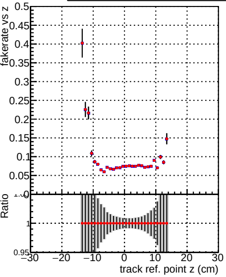
—•— DQM_TT_ORIGINAL —•— DQM_TT_MODIFIED_propToPlane_PRVersioniFINAL
