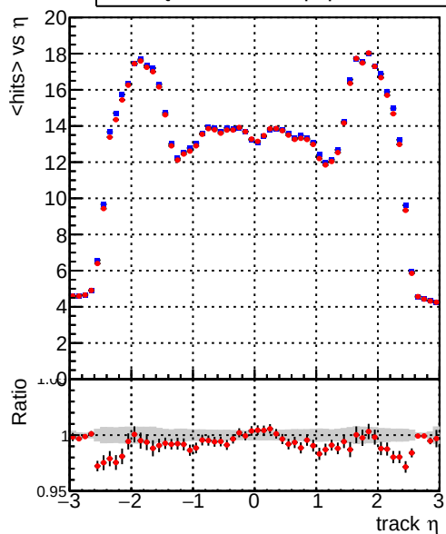
mean hits vs \eta Legend: DQM_TT_ORIGINAL (blue line), DQM_TT_MODIFIED_propToPlane_PRVersionFINAL (red line)
