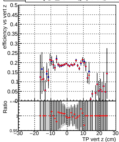
Efficiency vs. TP vert z (cm) — DQM_TT_ORIGINAL — DQM_TT_MODIFIED_propToPlane_PRRVersionFINAL
