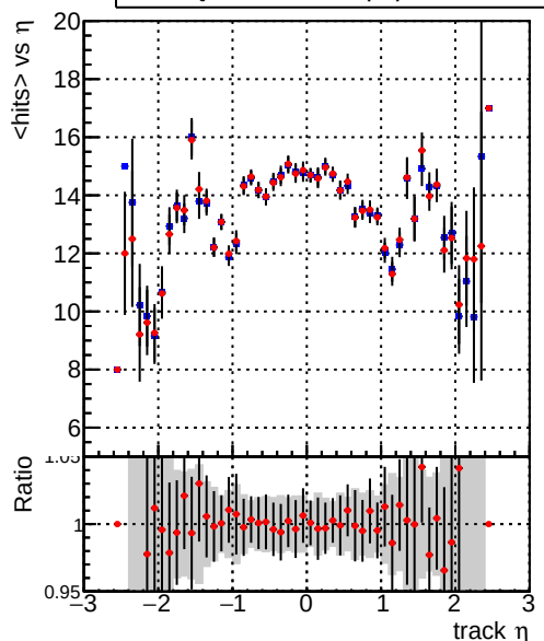
— DQM_TT_ORIGINAL — DQM_TT_MODIFIED_propToPlane_PRVersionFINAL mean hits
