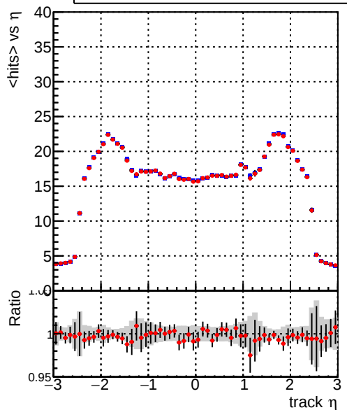
mean hits vs \eta — DQM_TT_ORIGINAL — DQM_TT_MODIFIED_propToPlane_PRVersionFINAL
