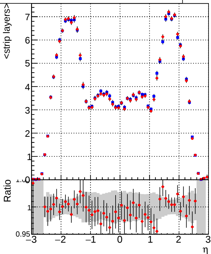
Legend: ■ DQM_TT_ORIGINAL ● DQM_TT_MODIFIED_propToPlane_PRVersioniFINAL
