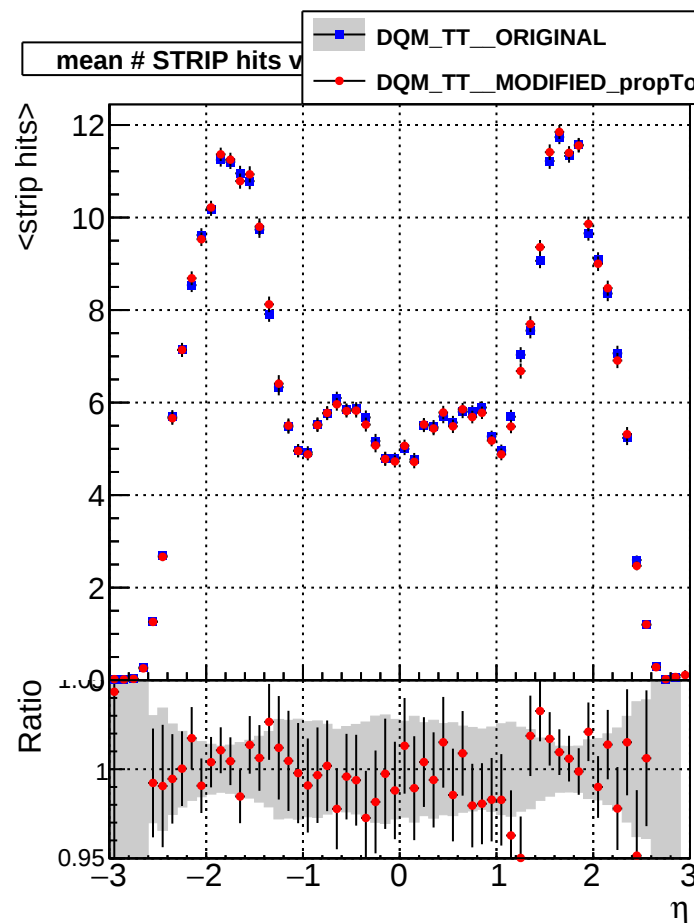
Legend: ■ DQM_TT_ORIGINAL ● DQM_TT_MODIFIED_propToPlane_PRVersioniFINAL
