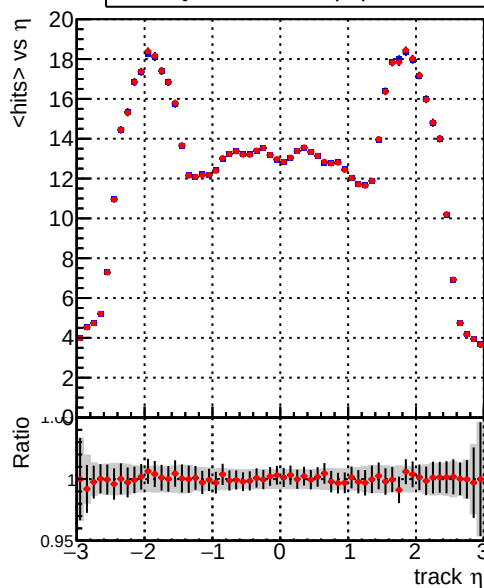
— DQM_TT_ORIGINAL — DQM_TT_MODIFIED_propToPlane_PRVersioniFINAL
