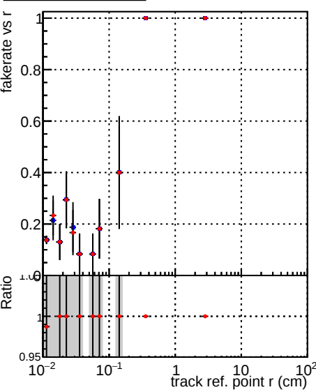
Fake rate vs verpos DQM_TT_ORIGINAL DQM_TT_MODIFIED_propToPlane_PRVersioniFINAL
