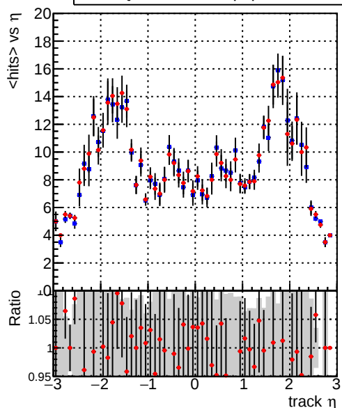
mean hits vs \eta Legend: DQM_TT_ORIGINAL (blue line with dots), DQM_TT_MODIFIED_propToPlane_PRVersionFINAL (red line with dots)
