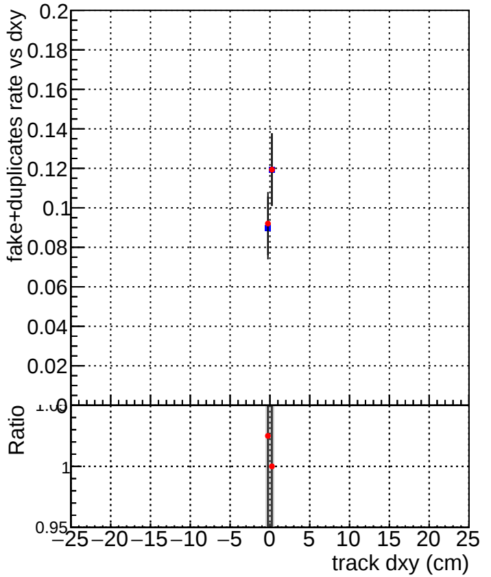
DQM_TT_ORIGINAL DQM_TT_MODIFIED_propToPlane_PRVersioniFINAL
