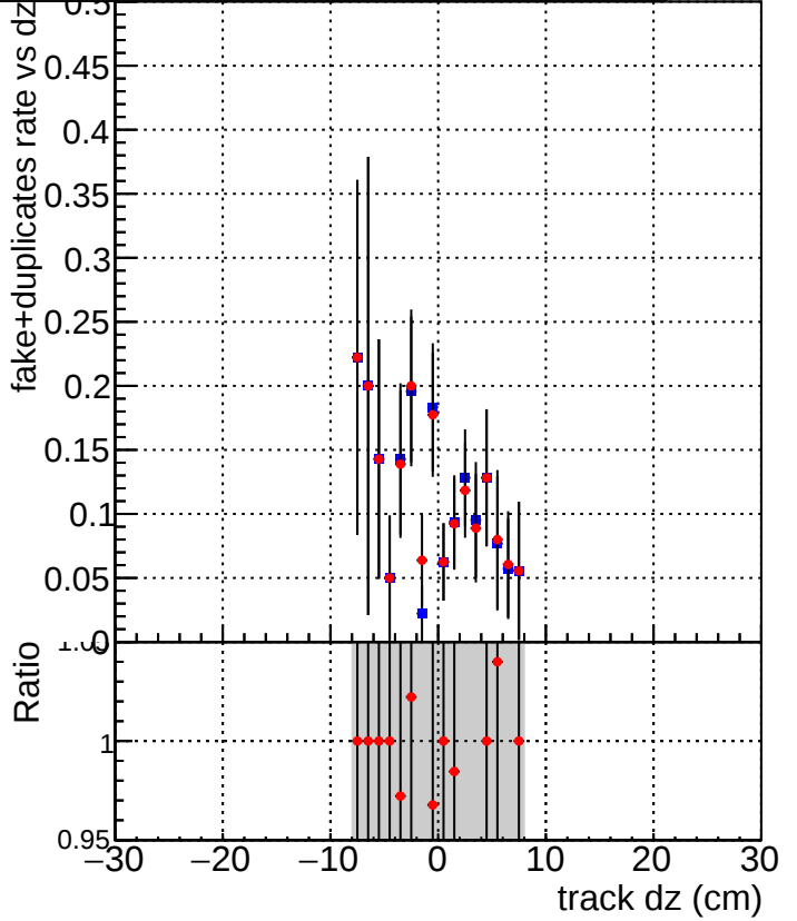
DQM_TT_ORIGINAL DQM_TT_MODIFIED_propToPlane_PRVersioniFINAL
