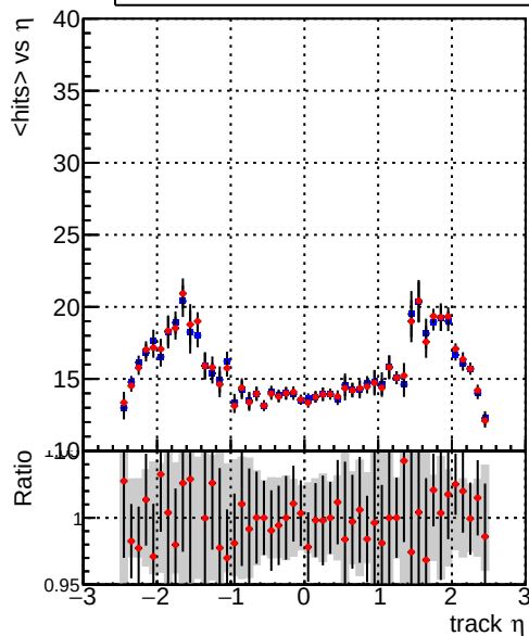
mean hit Legend: DQM_TT_ORIGINAL (blue line), DQM_TT_MODIFIED_propToPlane_PRVersioniFINAL (red line)
