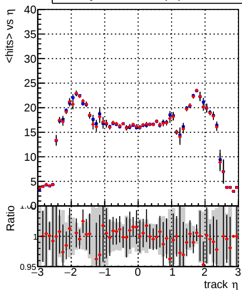
mean hit Legend: — DQM_TT_ORIGINAL — DQM_TT_MODIFIED_propToPlane_PRVersionFINAL
