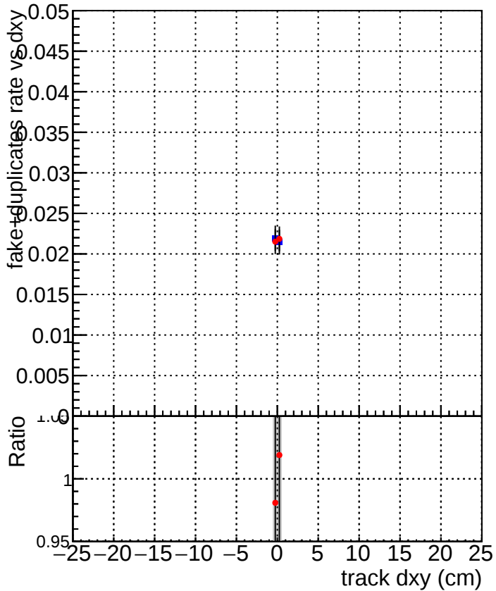
DQM_TT_ORIGINAL DQM_TT_MODIFIED_propToPlane_PRVersioniFINAL
