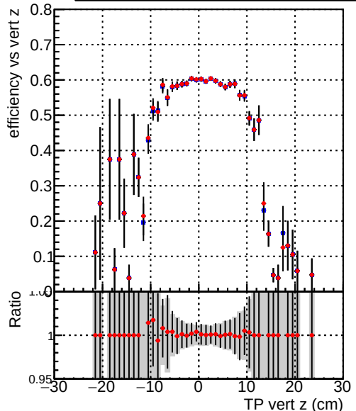
Efficiency vs TP vert z (cm) — DQM_TT_ORIGINAL (blue stars) — DQM_TT_MODIFIED_propToPlane_PVVersionFINAL (red stars)
