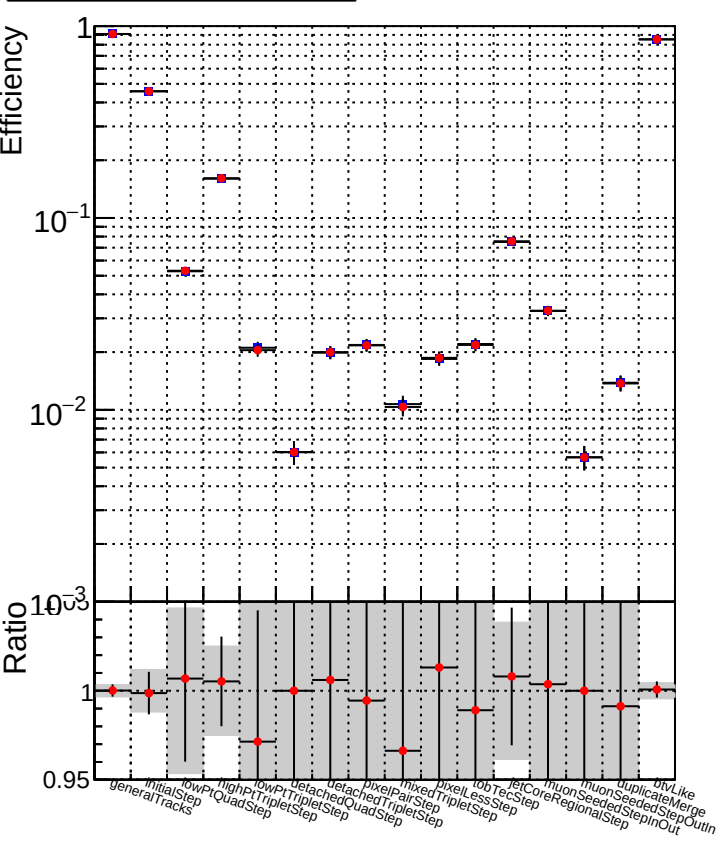
DQM_TT_ORIGINAL DQM_TT_MODIFIED_propToPlane_PRVersioniFINAL
